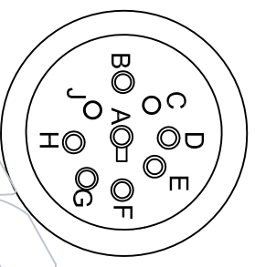
Caterpillar 9-Pin Male View A-A
